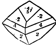
Greenovite.
